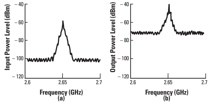
Figure 1-2. Typical signal and noise levels vs. frequency (a) at an amplifier's input and (b) at its output. Note that the noise level rises more than the signal level due to added noise from amplifier circuits. This relative rise in noise level is expressed by the amplifier noise figure.
